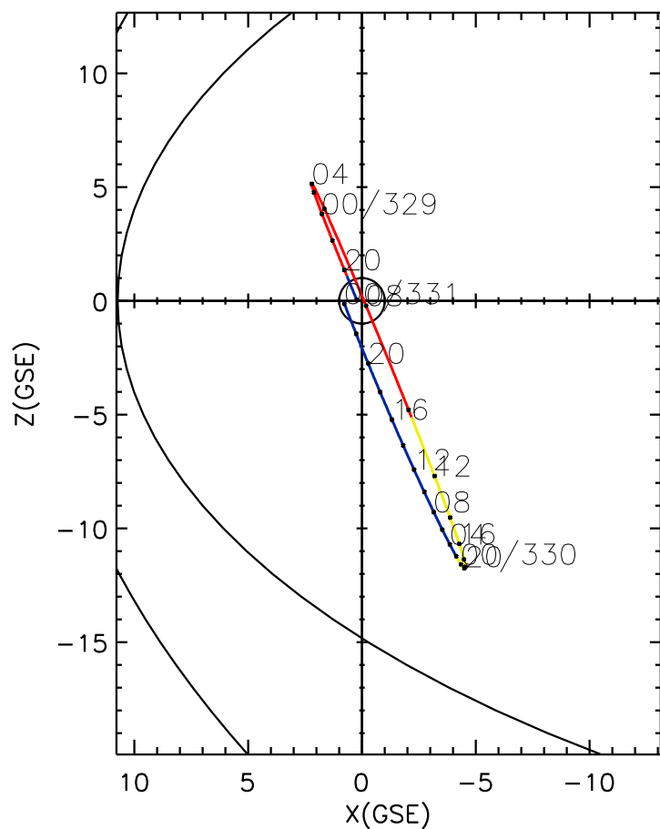
CLUSTER 2 orbit 2014 328 (11/24) 17:51 UT to 2014 331 (11/27) 00:11 UT
