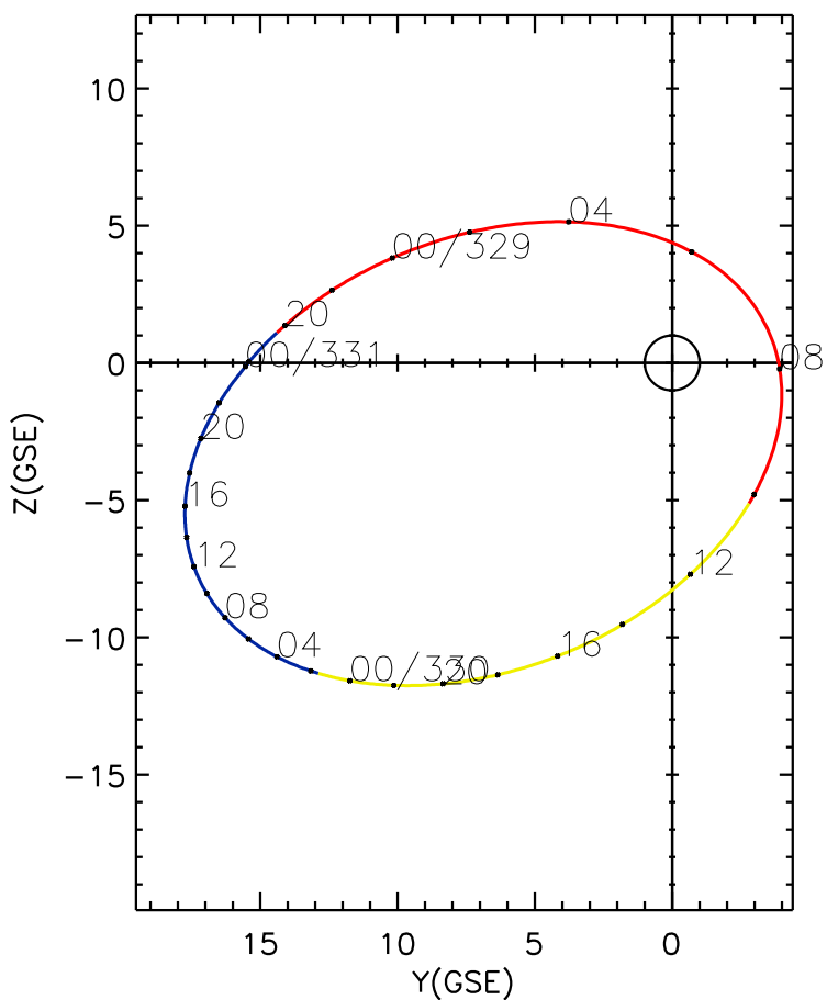
CLUSTER 2 orbit 2014 328 (11/24) 17:51 UT to 2014 331 (11/27) 00:11 UT
