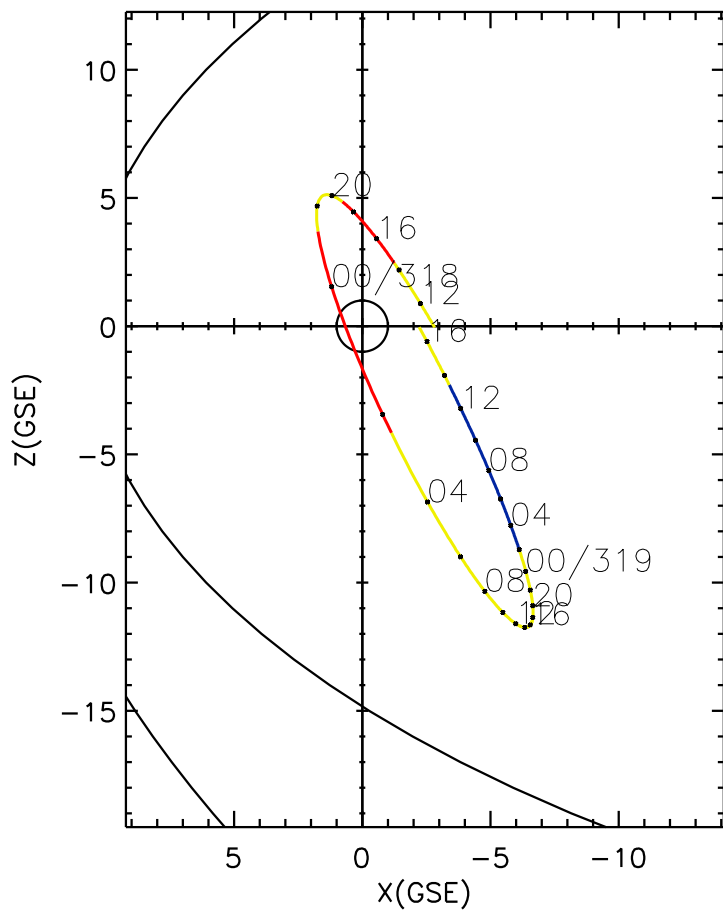
CLUSTER 2 orbit 2014 317 (11/13) 10:36 UT to 2014 319 (11/15) 16:51 UT
