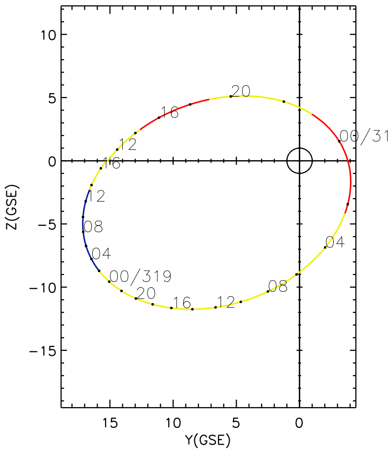
CLUSTER 2 orbit 2014 317 (11/13) 10:36 UT to 2014 319 (11/15) 16:51 UT
