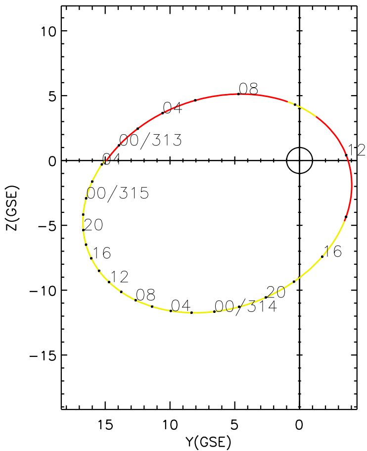
CLUSTER 2 orbit 2014 312 (11/08) 22:11 UT to 2014 315 (11/11) 04:26 UT
