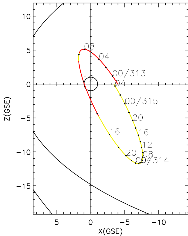
CLUSTER 2 orbit 2014 312 (11/08) 22:11 UT to 2014 315 (11/11) 04:26 UT
