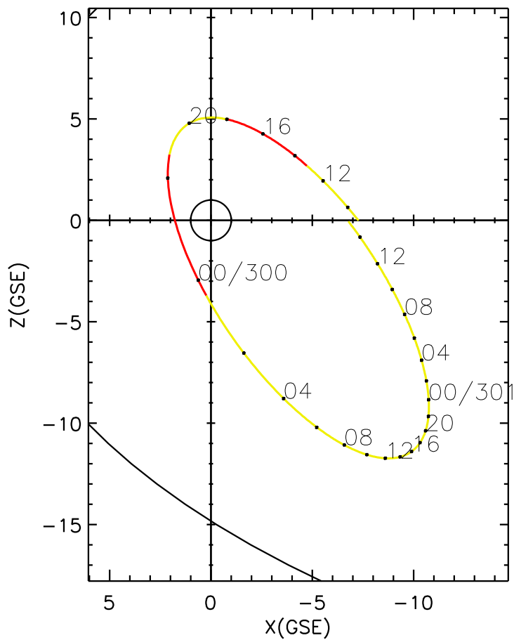
CLUSTER 2 orbit 2014 299 (10/26) 09:01 UT to 2014 301 (10/28) 15:11 UT
