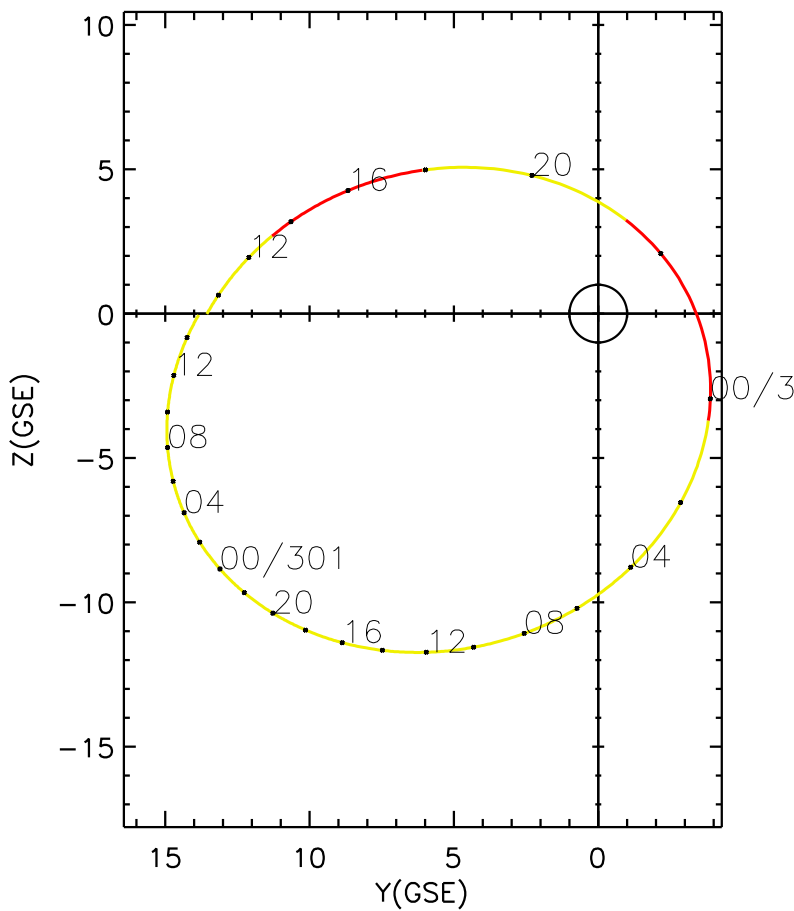
CLUSTER 2 orbit 2014 299 (10/26) 09:01 UT to 2014 301 (10/28) 15:11 UT
