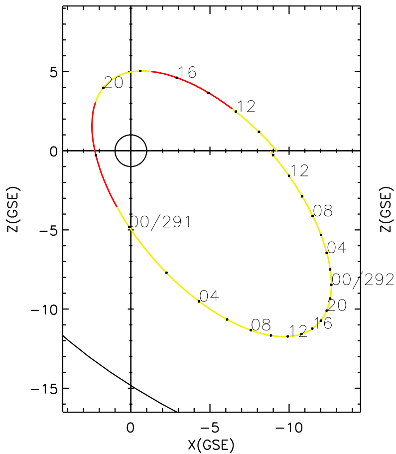
CLUSTER 2 orbit 2014 290 (10/17) 08:11 UT to 2014 292 (10/19) 14:21 UT
