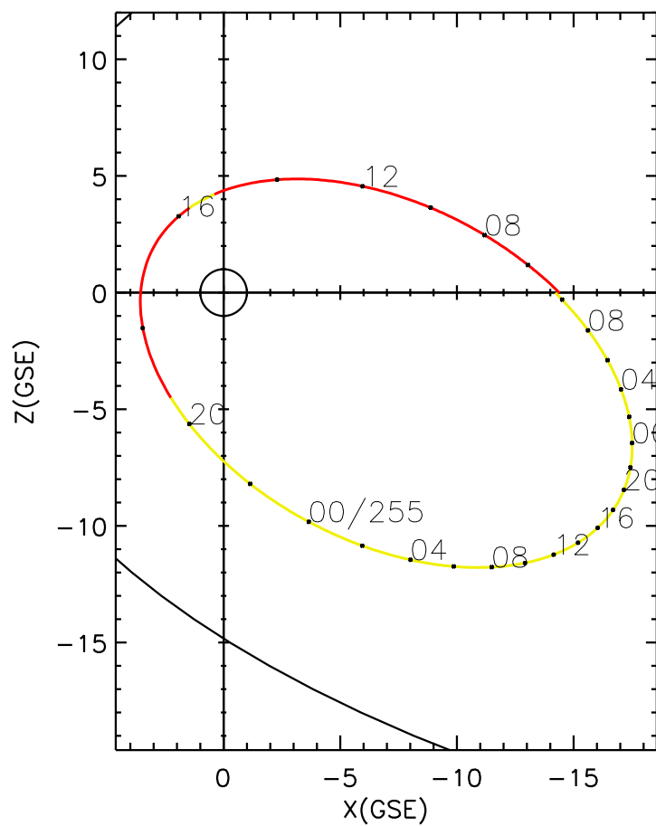
CLUSTER 2 orbit 2014 254 (09/11) 04:11 UT to 2014 256 (09/13) 10:26 UT
