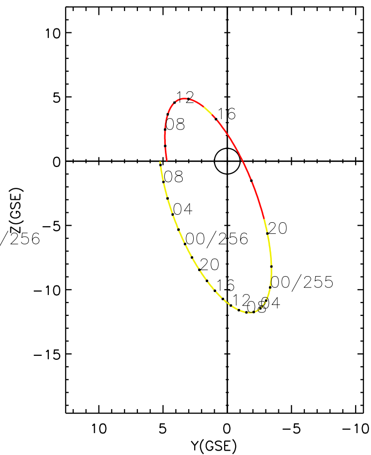
CLUSTER 2 orbit 2014 254 (09/11) 04:11 UT to 2014 256 (09/13) 10:26 UT
