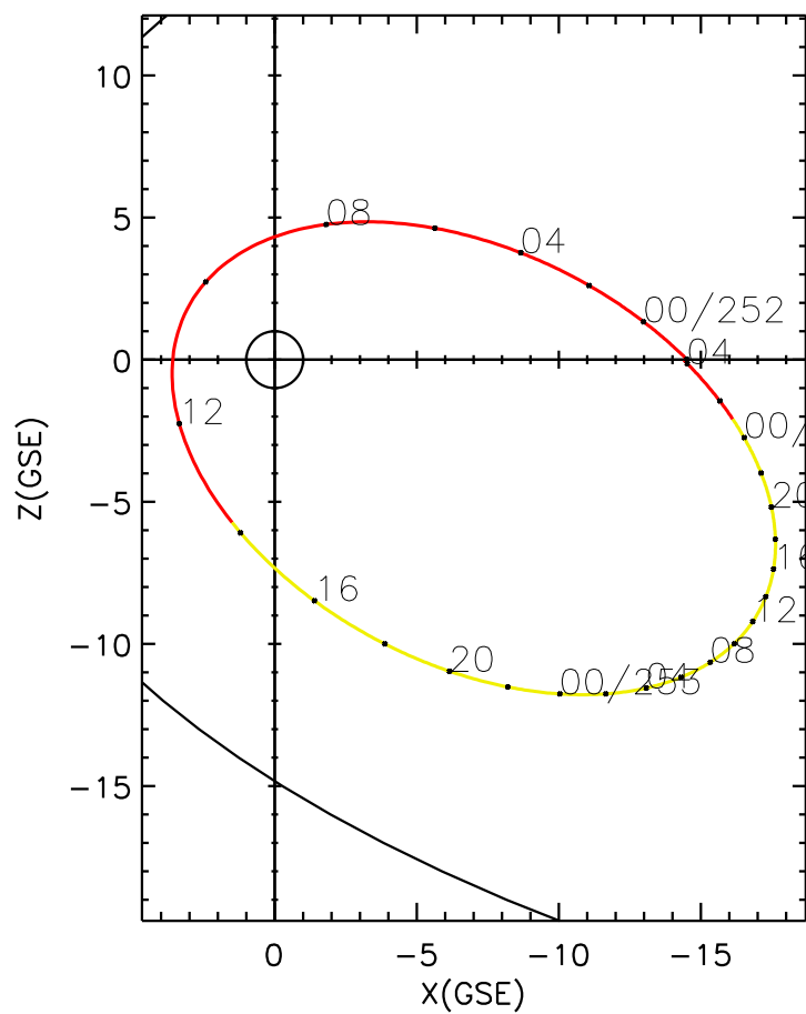
CLUSTER 2 orbit 2014 251 (09/08) 21:56 UT to 2014 254 (09/11) 04:11 UT
