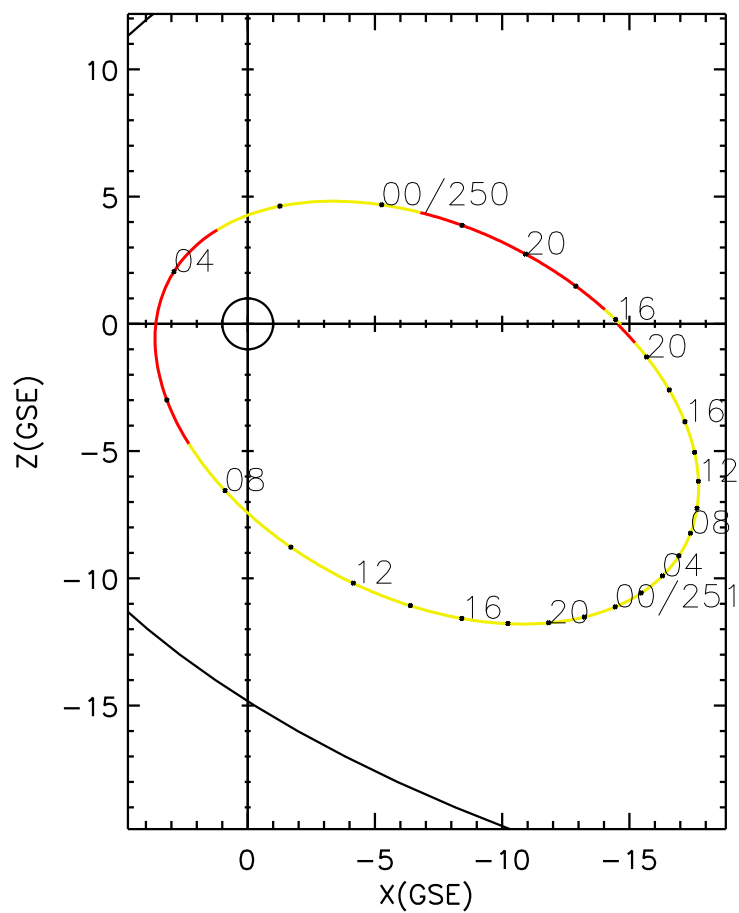
CLUSTER 2 orbit 2014 249 (09/06) 15:41 UT to 2014 251 (09/08) 21:56 UT
