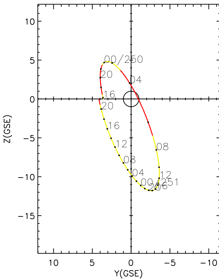
CLUSTER 2 orbit 2014 249 (09/06) 15:41 UT to 2014 251 (09/08) 21:56 UT
