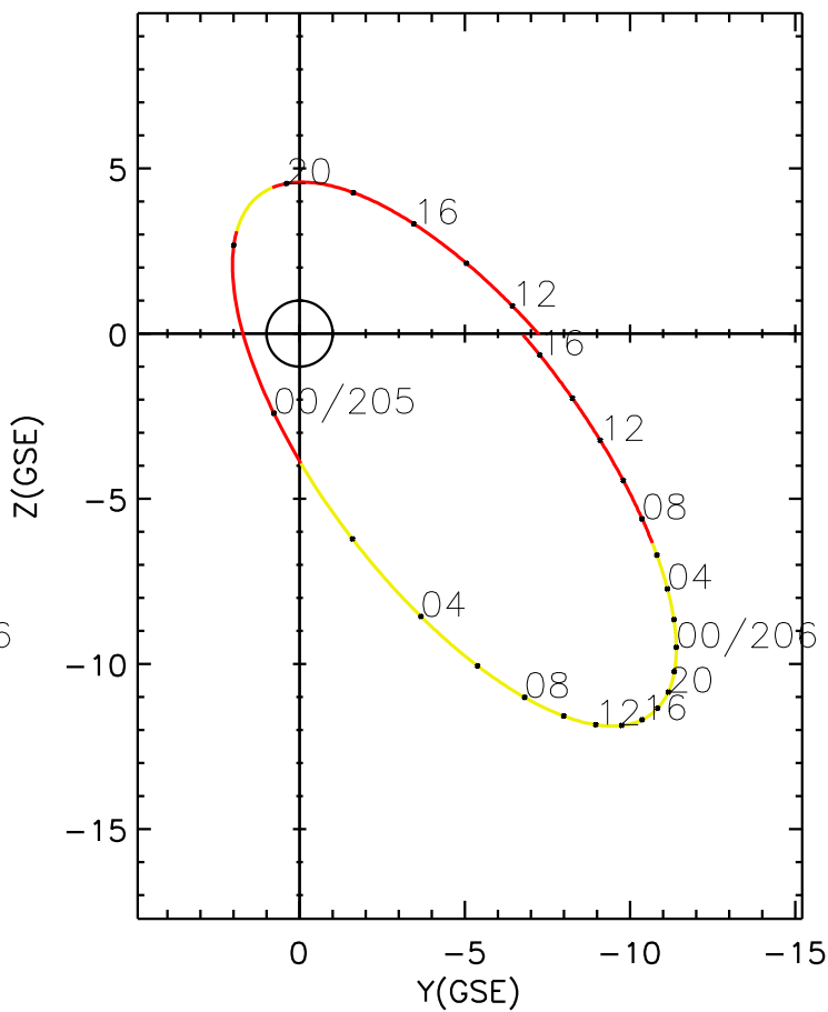
CLUSTER 2 orbit 2014 204 (07/23) 10:41 UT to 2014 206 (07/25) 16:56 UT
