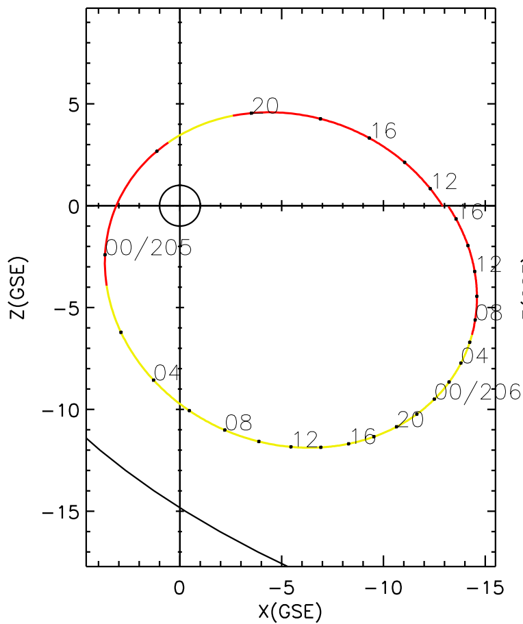
CLUSTER 2 orbit 2014 204 (07/23) 10:41 UT to 2014 206 (07/25) 16:56 UT
