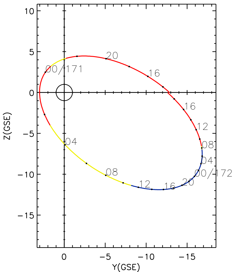
CLUSTER 2 orbit 2014 170 (06/19) 12:56 UT to 2014 172 (06/21) 19:11 UT
