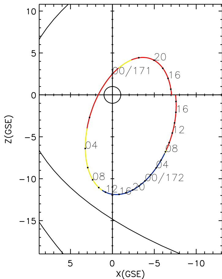
CLUSTER 2 orbit 2014 170 (06/19) 12:56 UT to 2014 172 (06/21) 19:11 UT
