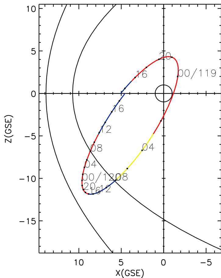
CLUSTER 2 orbit 2014 118 (04/28) 13:01 UT to 2014 120 (04/30) 19:16 UT
