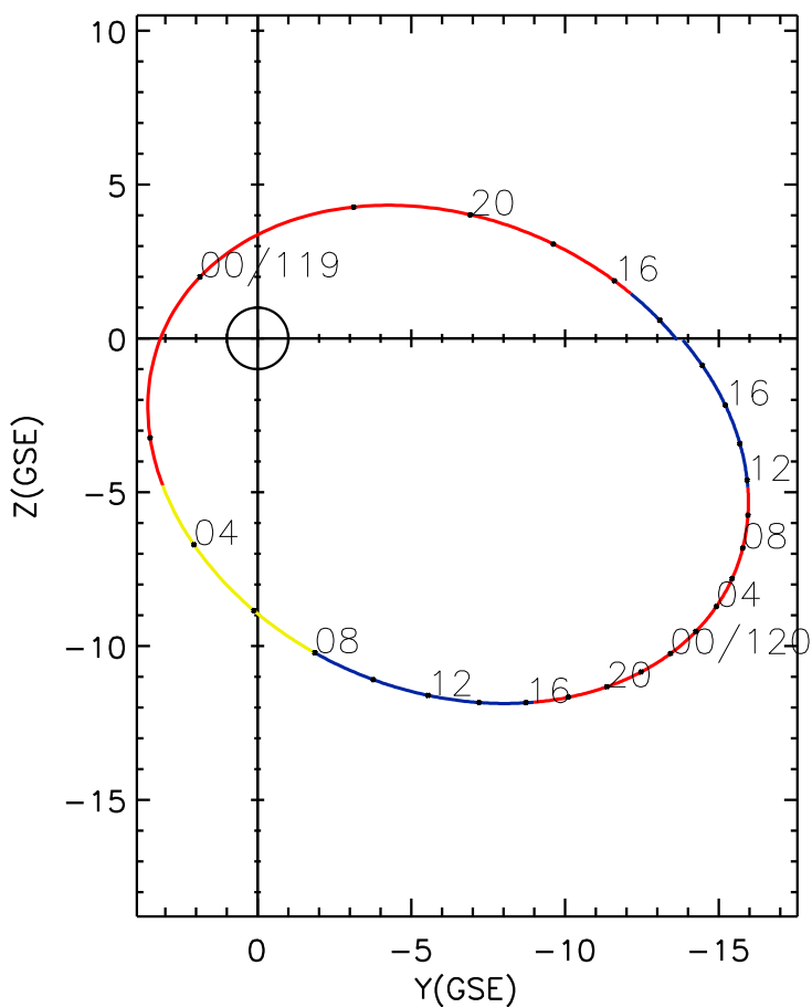
CLUSTER 2 orbit 2014 118 (04/28) 13:01 UT to 2014 120 (04/30) 19:16 UT
