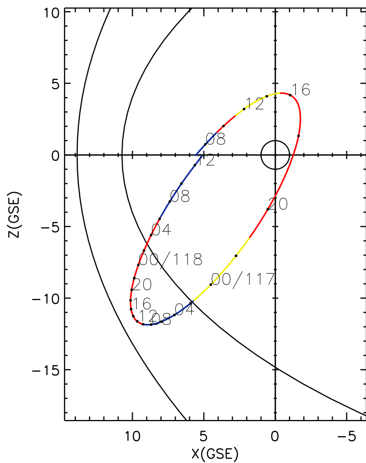
CLUSTER 2 orbit 2014 116 (04/26) 06:46 UT to 2014 118 (04/28) 13:01 UT
