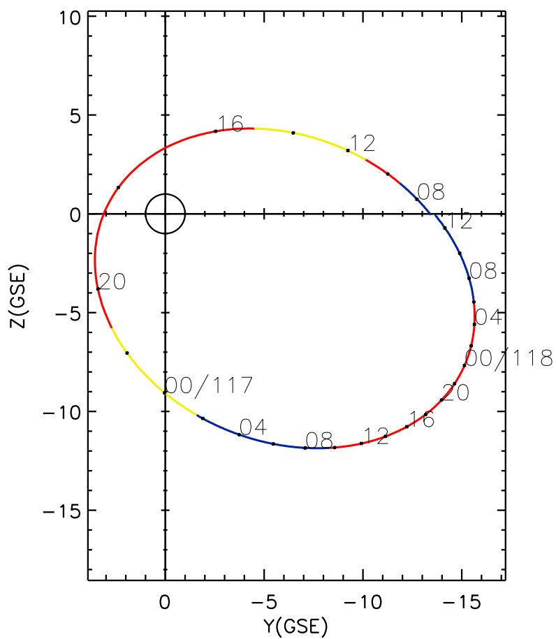
CLUSTER 2 orbit 2014 116 (04/26) 06:46 UT to 2014 118 (04/28) 13:01 UT
