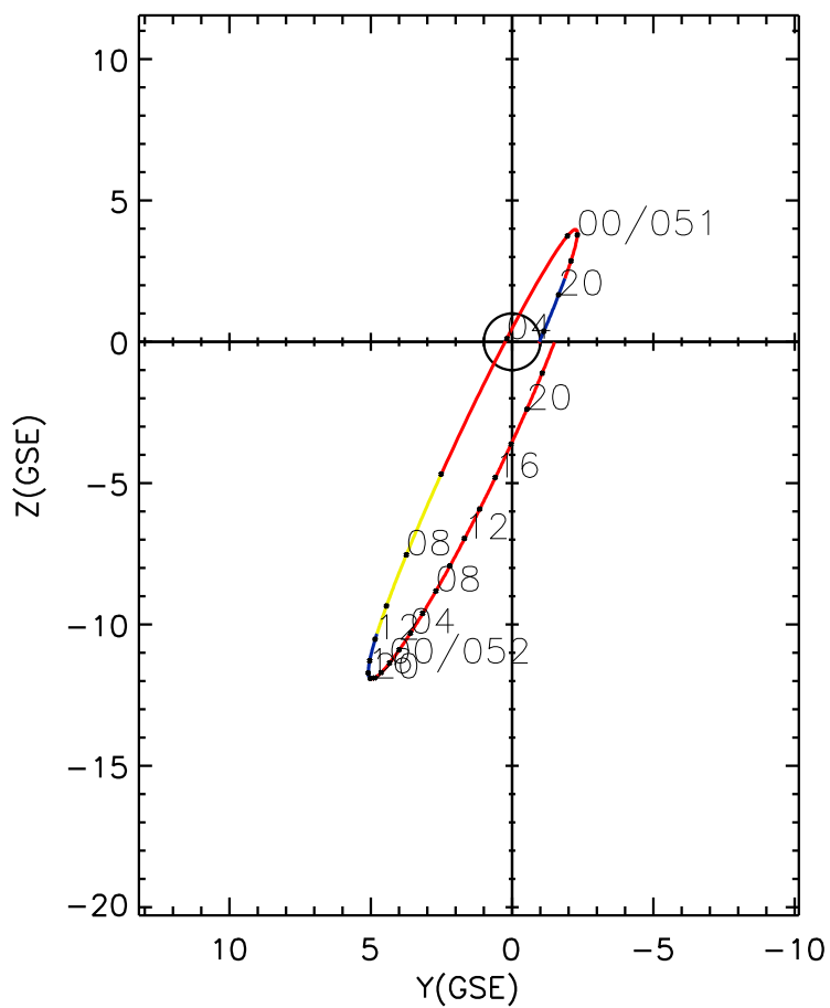
CLUSTER 2 orbit 2014 050 (02/19) 17:21 UT to 2014 052 (02/21) 23:41 UT
