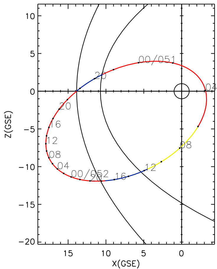
CLUSTER 2 orbit 2014 050 (02/19) 17:21 UT to 2014 052 (02/21) 23:41 UT
