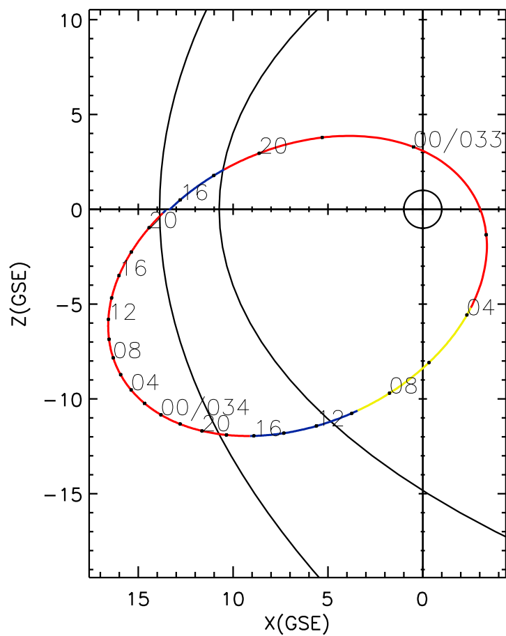
CLUSTER 2 orbit 2014 032 (02/01) 15:11 UT to 2014 034 (02/03) 21:26 UT
