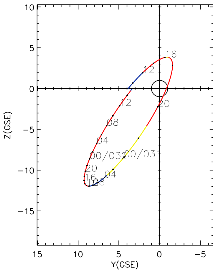
CLUSTER 2 orbit 2014 030 (01/30) 08:56 UT to 2014 032 (02/01) 15:11 UT
