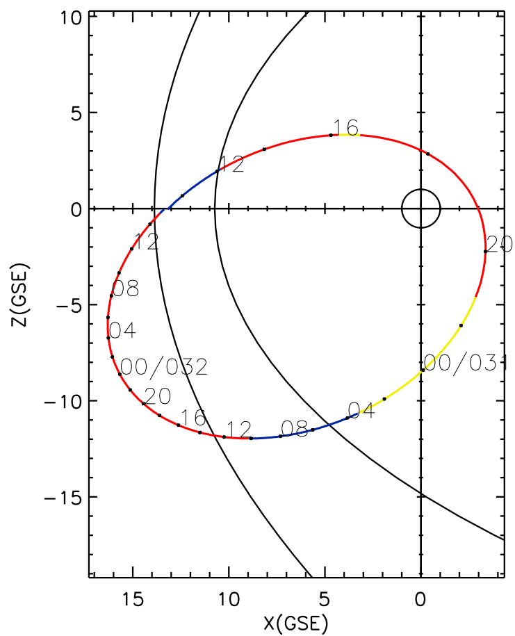
CLUSTER 2 orbit 2014 030 (01/30) 08:56 UT to 2014 032 (02/01) 15:11 UT
