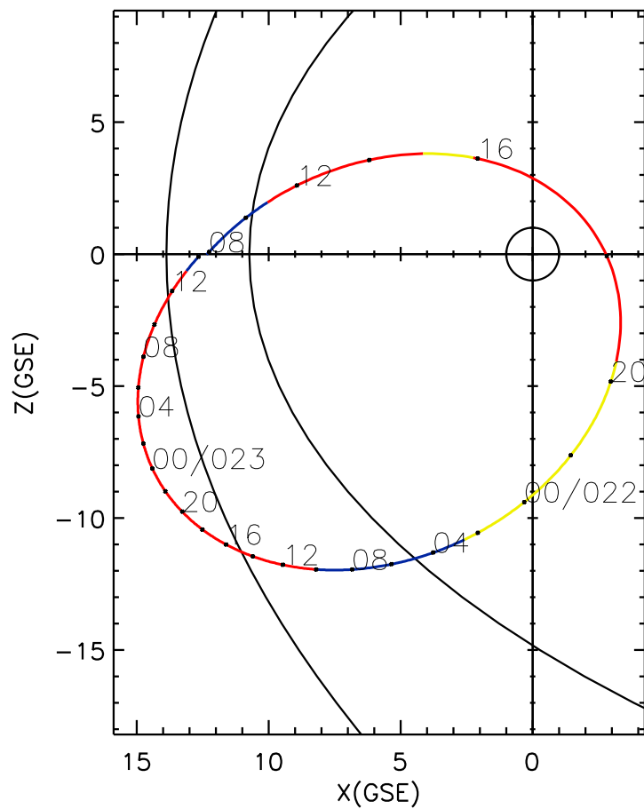
CLUSTER 2 orbit 2014 021 (01/21) 07:51 UT to 2014 023 (01/23) 14:06 UT
