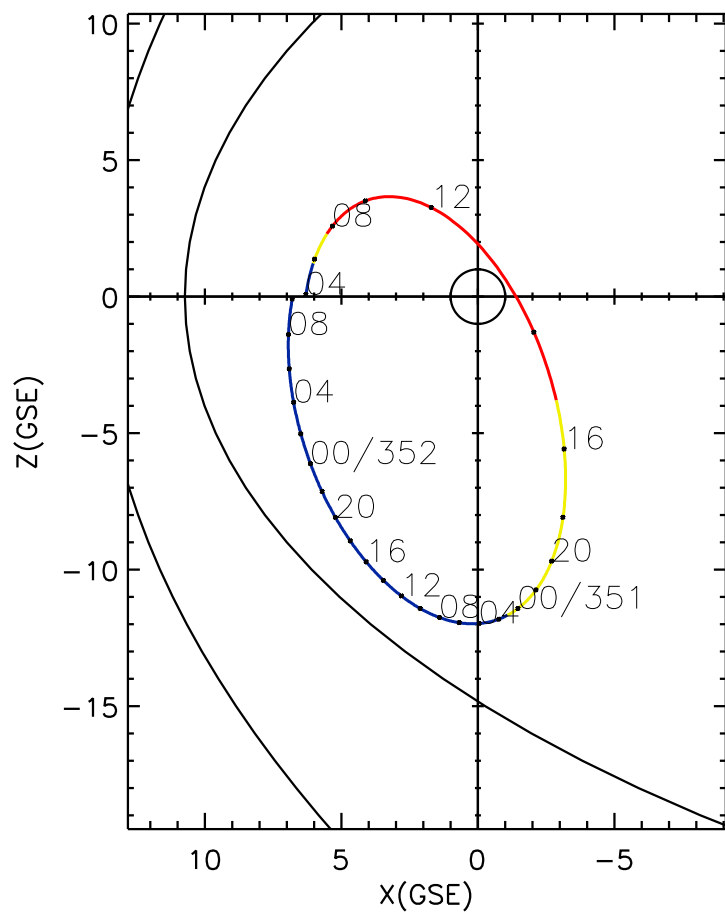
CLUSTER 2 orbit 2013 350 (12/16) 03:51 UT to 2013 352 (12/18) 10:06 UT
