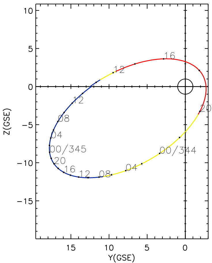
CLUSTER 2 orbit 2013 343 (12/09) 09:06 UT to 2013 345 (12/11) 15:21 UT
