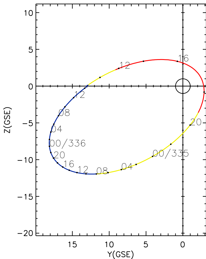
CLUSTER 2 orbit 2013 334 (11/30) 08:06 UT to 2013 336 (12/02) 14:21 UT
