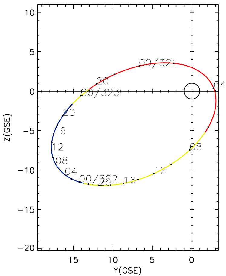
CLUSTER 2 orbit 2013 320 (11/16) 18:36 UT to 2013 323 (11/19) 00:51 UT
