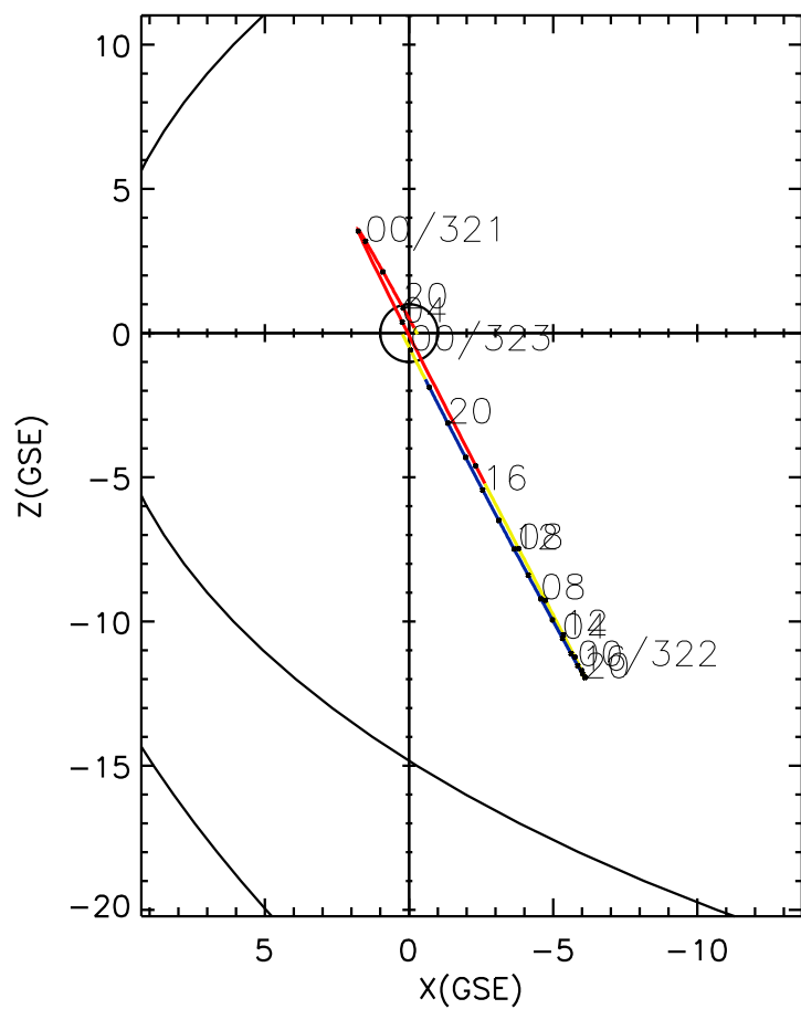
CLUSTER 2 orbit 2013 320 (11/16) 18:36 UT to 2013 323 (11/19) 00:51 UT
