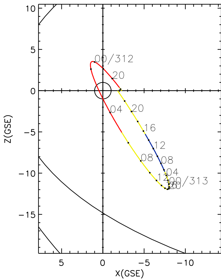
CLUSTER 2 orbit 2013 311 (11/07) 17:41 UT to 2013 313 (11/09) 23:56 UT
