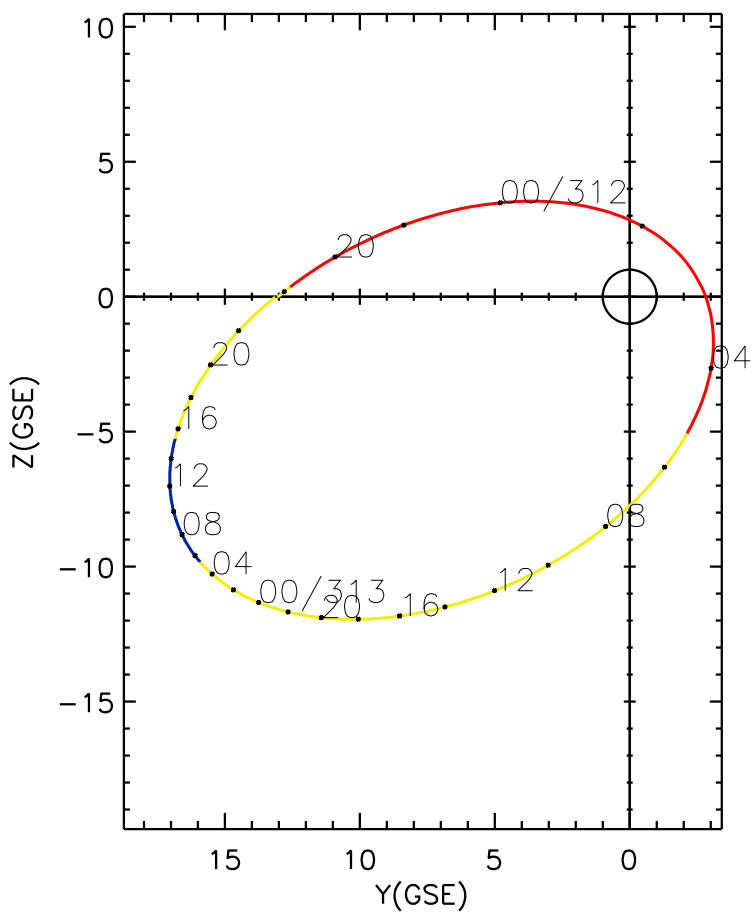
CLUSTER 2 orbit 2013 311 (11/07) 17:41 UT to 2013 313 (11/09) 23:56 UT
