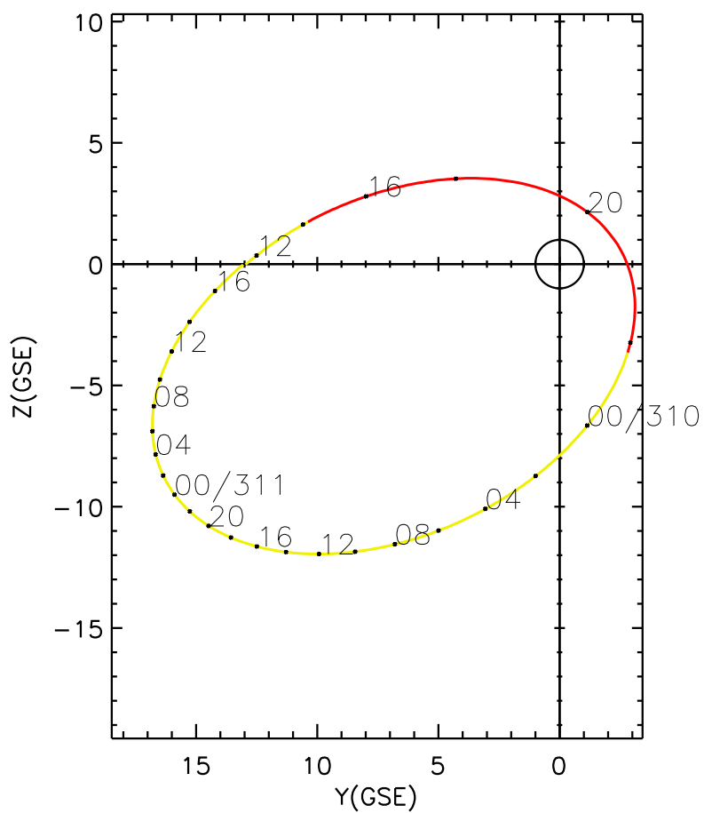
CLUSTER 2 orbit 2013 309 (11/05) 11:26 UT to 2013 311 (11/07) 17:41 UT
