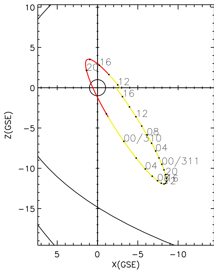
CLUSTER 2 orbit 2013 309 (11/05) 11:26 UT to 2013 311 (11/07) 17:41 UT
