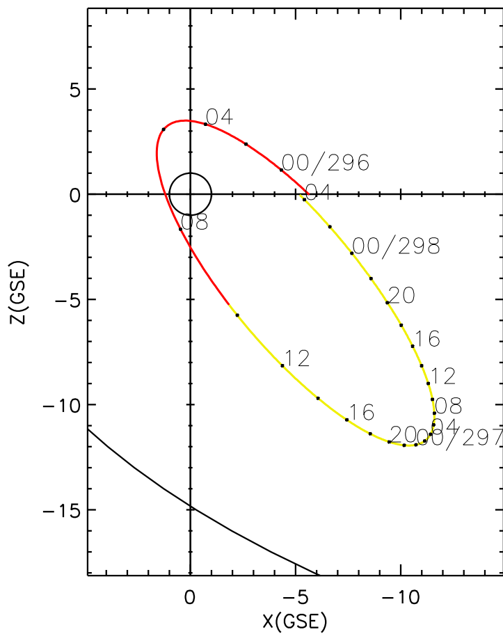
CLUSTER 2 orbit 2013 295 (10/22) 22:11 UT to 2013 298 (10/25) 04:21 UT
