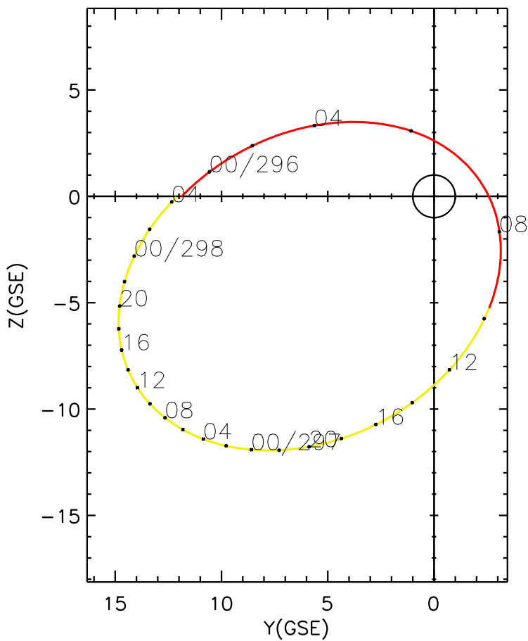
CLUSTER 2 orbit 2013 295 (10/22) 22:11 UT to 2013 298 (10/25) 04:21 UT
