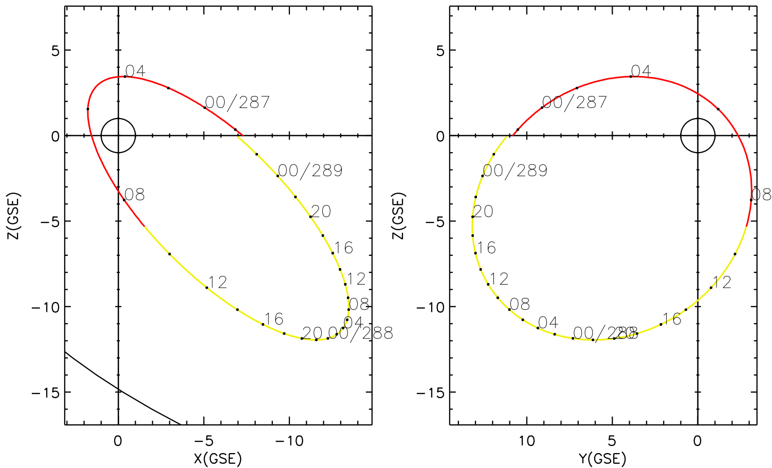
CLUSTER 2 orbit 2013 286 (10/13) 21:26 UT to 2013 289 (10/16) 03:36 UT
