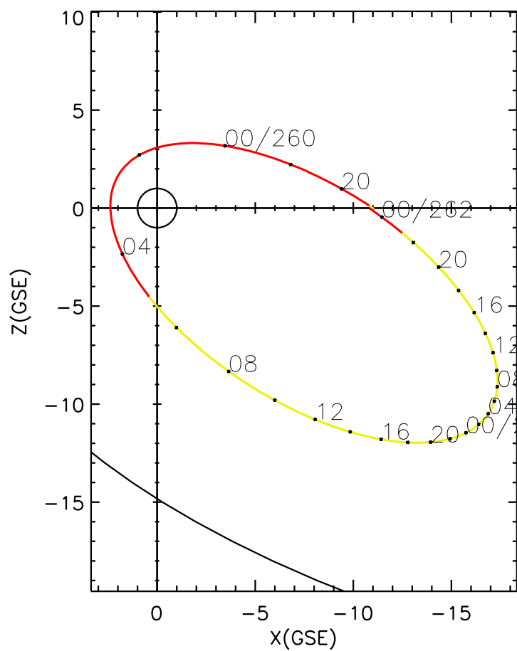
CLUSTER 2 orbit 2013 259 (09/16) 18:26 UT to 2013 262 (09/19) 00:41 UT
