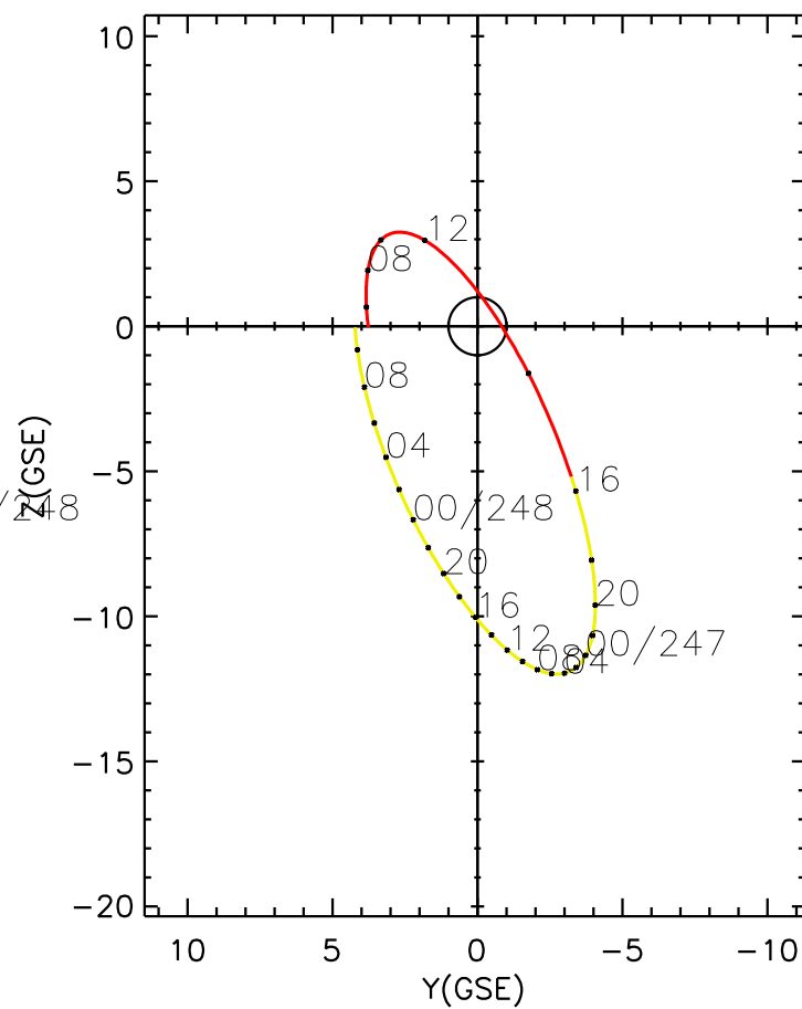
CLUSTER 2 orbit 2013 246 (09/03) 04:56 UT to 2013 248 (09/05) 11:11 UT
