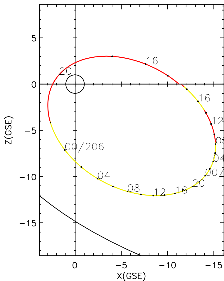
CLUSTER 2 orbit 2013 205 (07/24) 12:36 UT to 2013 207 (07/26) 18:46 UT
