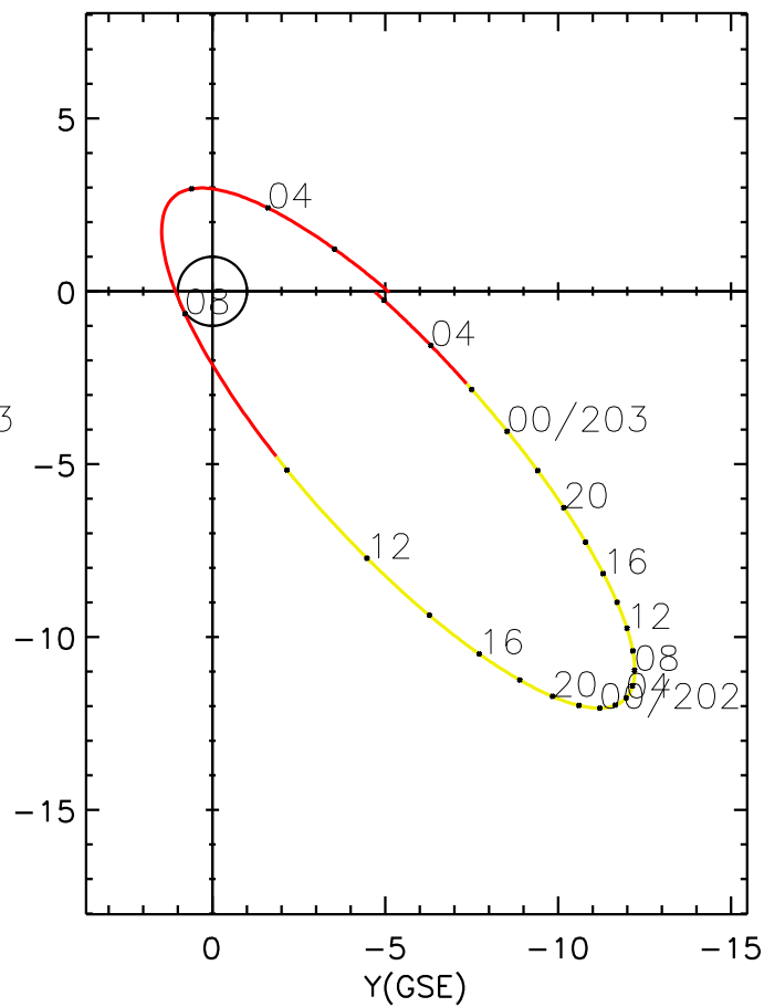
CLUSTER 2 orbit 2013 201 (07/20) 00:06 UT to 2013 203 (07/22) 06:21 UT
