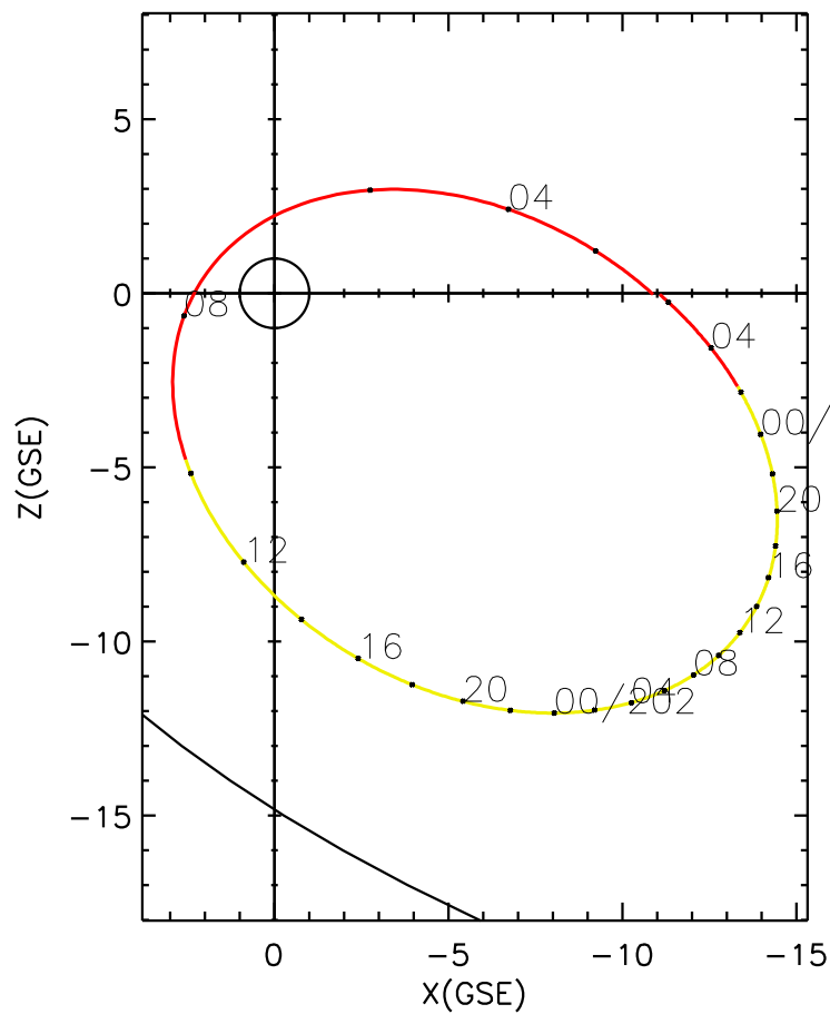
CLUSTER 2 orbit 2013 201 (07/20) 00:06 UT to 2013 203 (07/22) 06:21 UT
