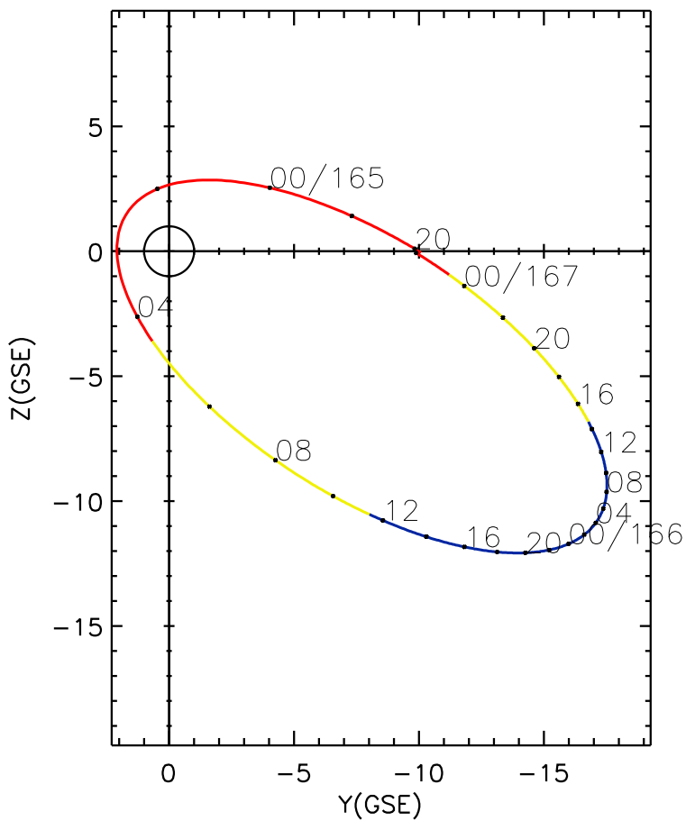
CLUSTER 2 orbit 2013 164 (06/13) 19:46 UT to 2013 167 (06/16) 02:01 UT
