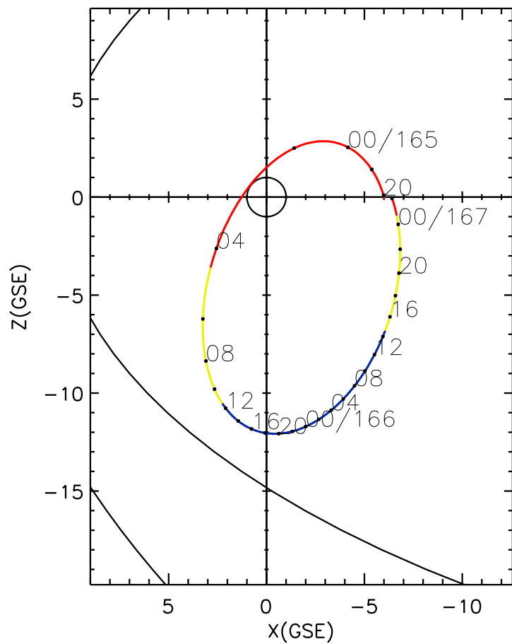
CLUSTER 2 orbit 2013 164 (06/13) 19:46 UT to 2013 167 (06/16) 02:01 UT
