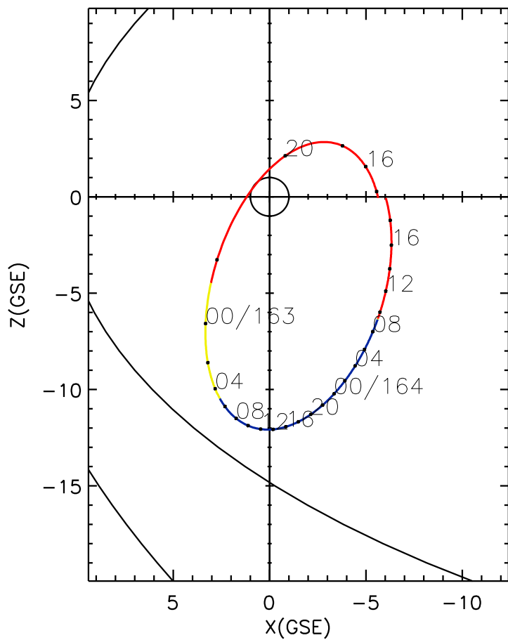
CLUSTER 2 orbit 2013 162 (06/11) 13:31 UT to 2013 164 (06/13) 19:46 UT
