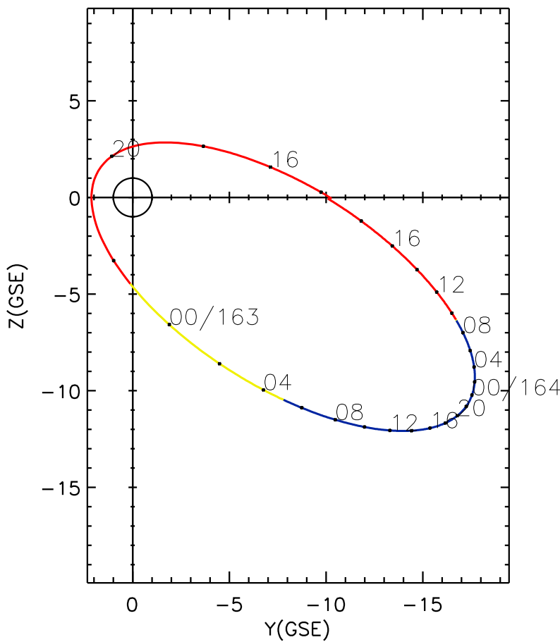
CLUSTER 2 orbit 2013 162 (06/11) 13:31 UT to 2013 164 (06/13) 19:46 UT
