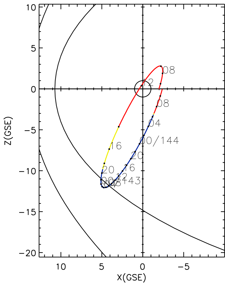
CLUSTER 2 orbit 2013 142 (05/22) 05:01 UT to 2013 144 (05/24) 11:16 UT
