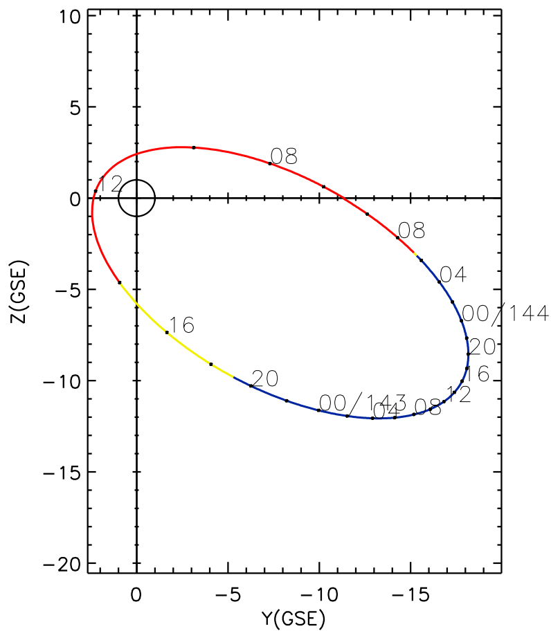
CLUSTER 2 orbit 2013 142 (05/22) 05:01 UT to 2013 144 (05/24) 11:16 UT
