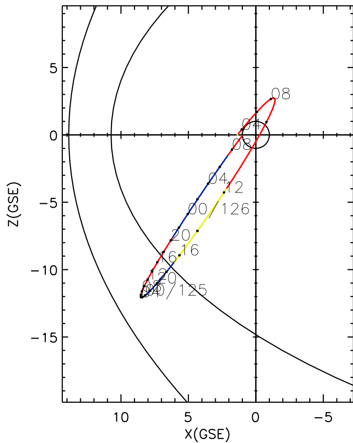
CLUSTER 2 orbit 2013 124 (05/04) 03:21 UT to 2013 126 (05/06) 09:36 UT
