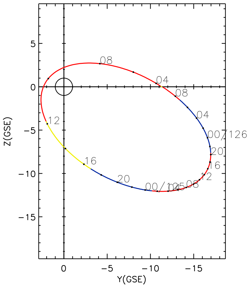
CLUSTER 2 orbit 2013 124 (05/04) 03:21 UT to 2013 126 (05/06) 09:36 UT
