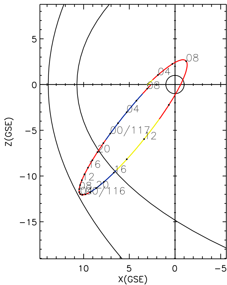
CLUSTER 2 orbit 2013 115 (04/25) 02:21 UT to 2013 117 (04/27) 08:36 UT
