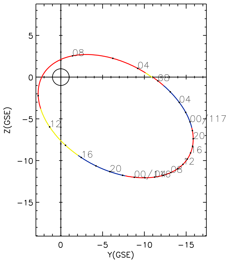
CLUSTER 2 orbit 2013 115 (04/25) 02:21 UT to 2013 117 (04/27) 08:36 UT
