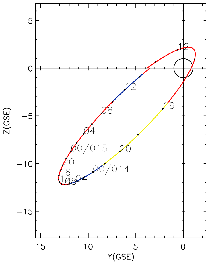
CLUSTER 2 orbit 2013 013 (01/13) 09:01 UT to 2013 015 (01/15) 15:16 UT
