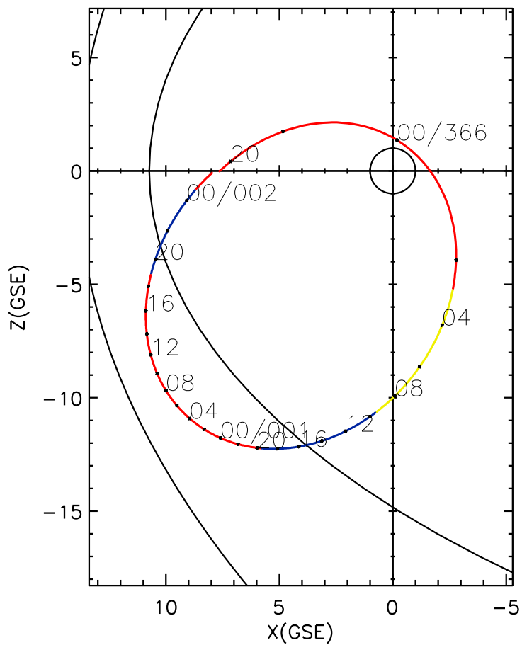
CLUSTER 2 orbit 2012 365 (12/30) 19:21 UT to 2013 002 (01/02) 01:46 UT
