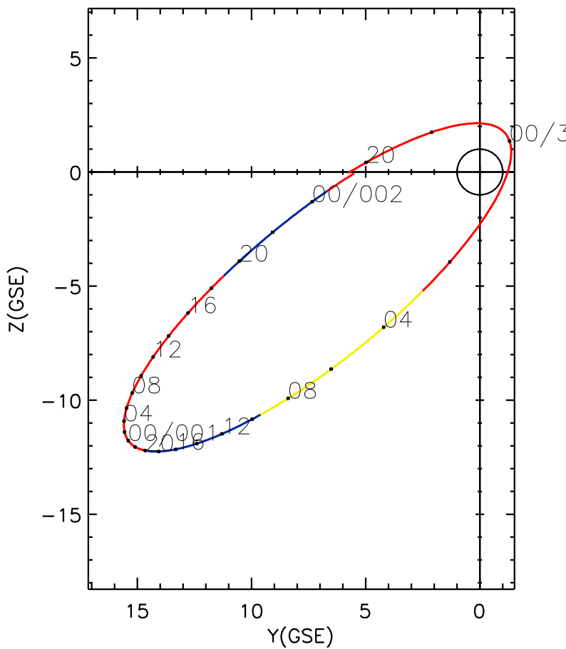
CLUSTER 2 orbit 2012 365 (12/30) 19:21 UT to 2013 002 (01/02) 01:46 UT
