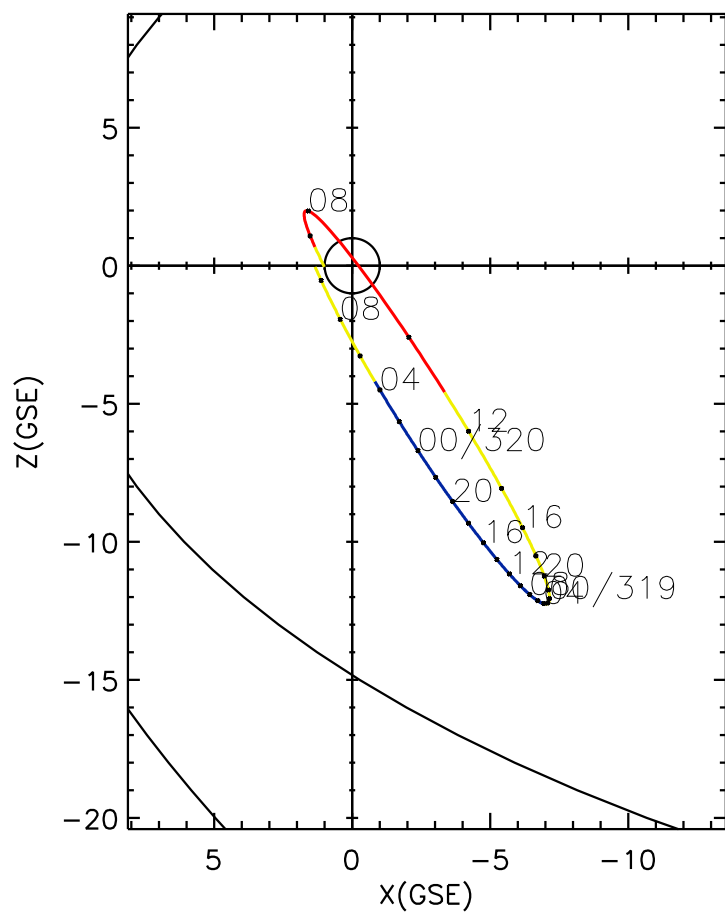
CLUSTER 2 orbit 2012 318 (11/13) 04:26 UT to 2012 320 (11/15) 10:41 UT
