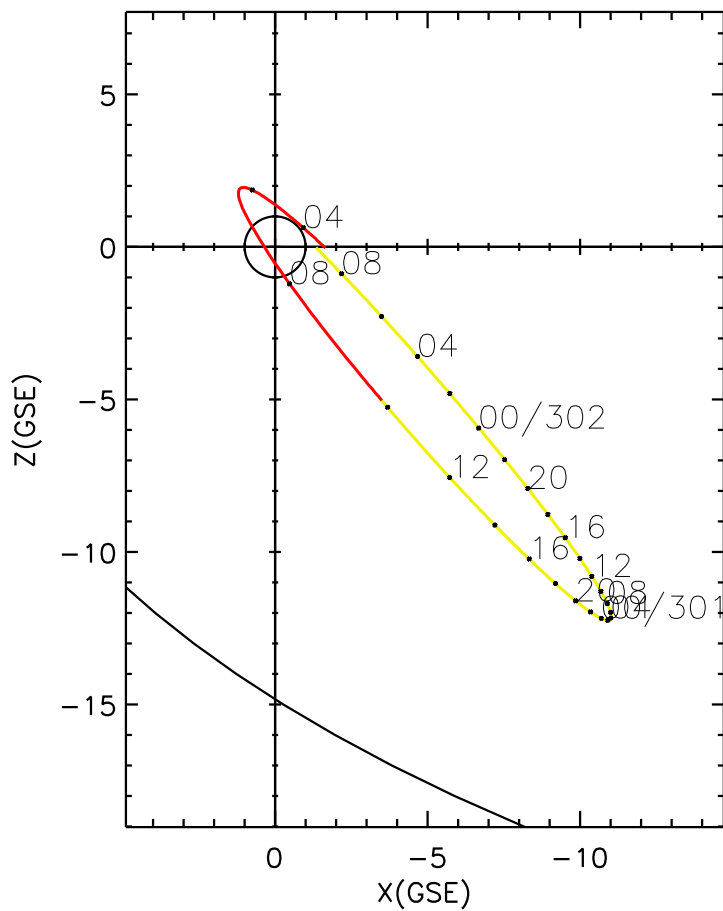
CLUSTER 2 orbit 2012 300 (10/26) 03:06 UT to 2012 302 (10/28) 09:11 UT
