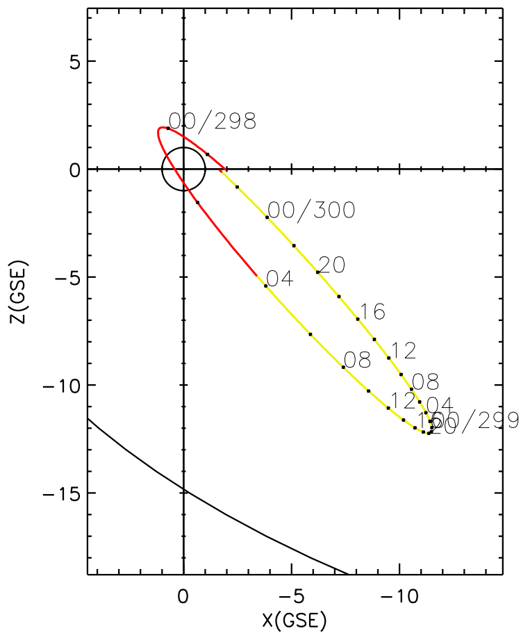
CLUSTER 2 orbit 2012 297 (10/23) 21:01 UT to 2012 300 (10/26) 03:06 UT
