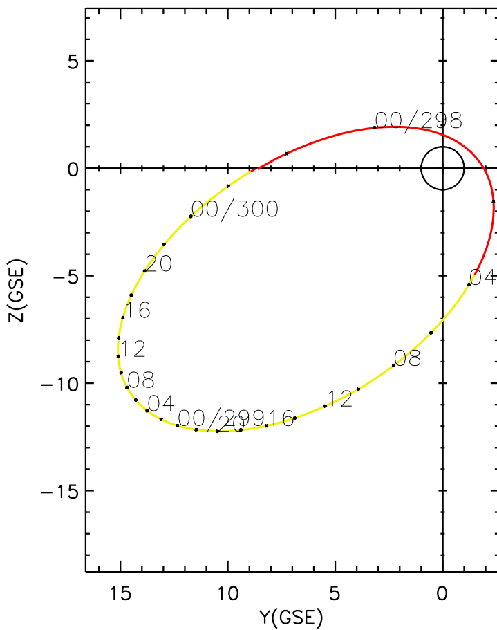
CLUSTER 2 orbit 2012 297 (10/23) 21:01 UT to 2012 300 (10/26) 03:06 UT
