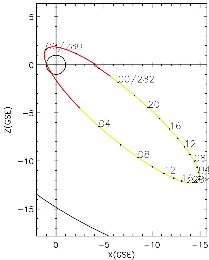
CLUSTER 2 orbit 2012 279 (10/05) 20:21 UT to 2012 282 (10/08) 02:26 UT
