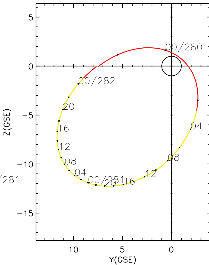
CLUSTER 2 orbit 2012 279 (10/05) 20:21 UT to 2012 282 (10/08) 02:26 UT
