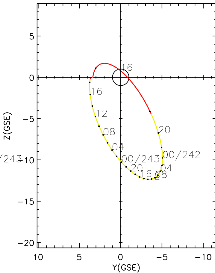
CLUSTER 2 orbit 2012 241 (08/28) 12:31 UT to 2012 243 (08/30) 18:46 UT
