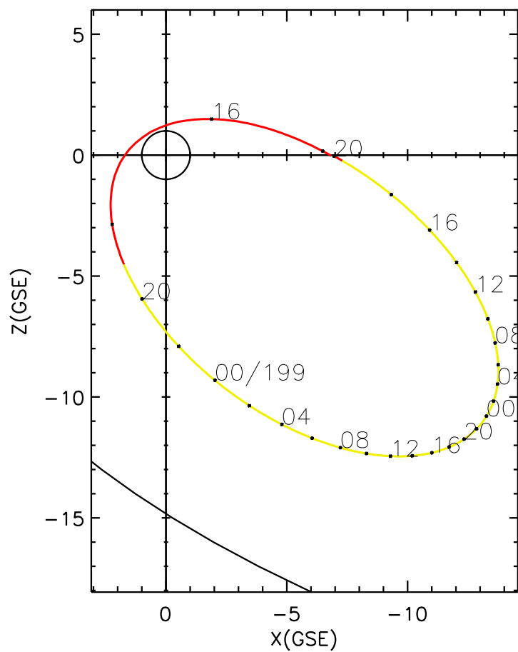
CLUSTER 2 orbit 2012 198 (07/16) 13:46 UT to 2012 200 (07/18) 20:01 UT
