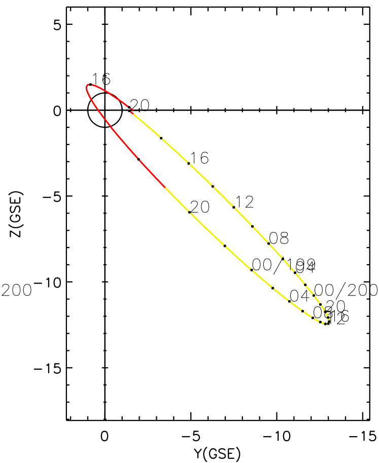
CLUSTER 2 orbit 2012 198 (07/16) 13:46 UT to 2012 200 (07/18) 20:01 UT
