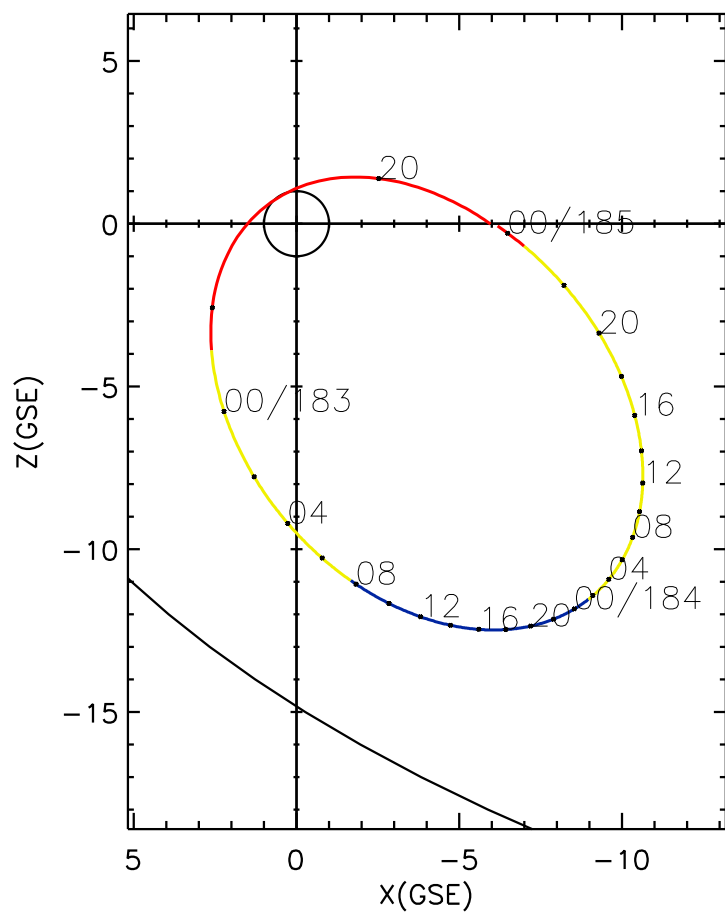
CLUSTER 2 orbit 2012 182 (06/30) 18:06 UT to 2012 185 (07/03) 00:16 UT
