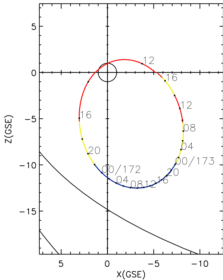
CLUSTER 2 orbit 2012 171 (06/19) 10:46 UT to 2012 173 (06/21) 17:01 UT
