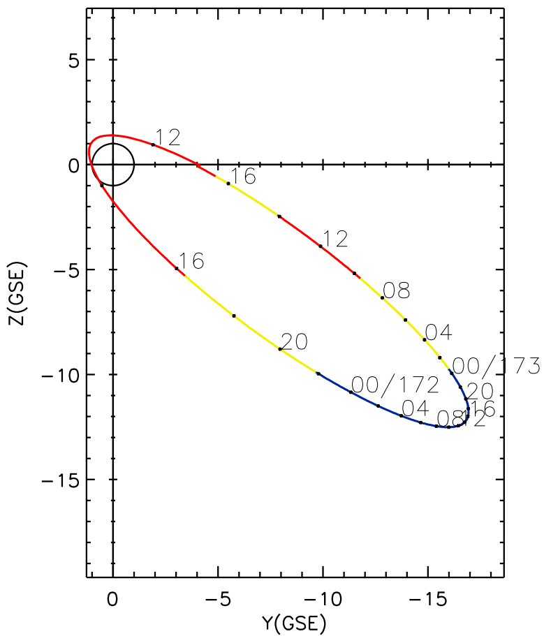
CLUSTER 2 orbit 2012 171 (06/19) 10:46 UT to 2012 173 (06/21) 17:01 UT
