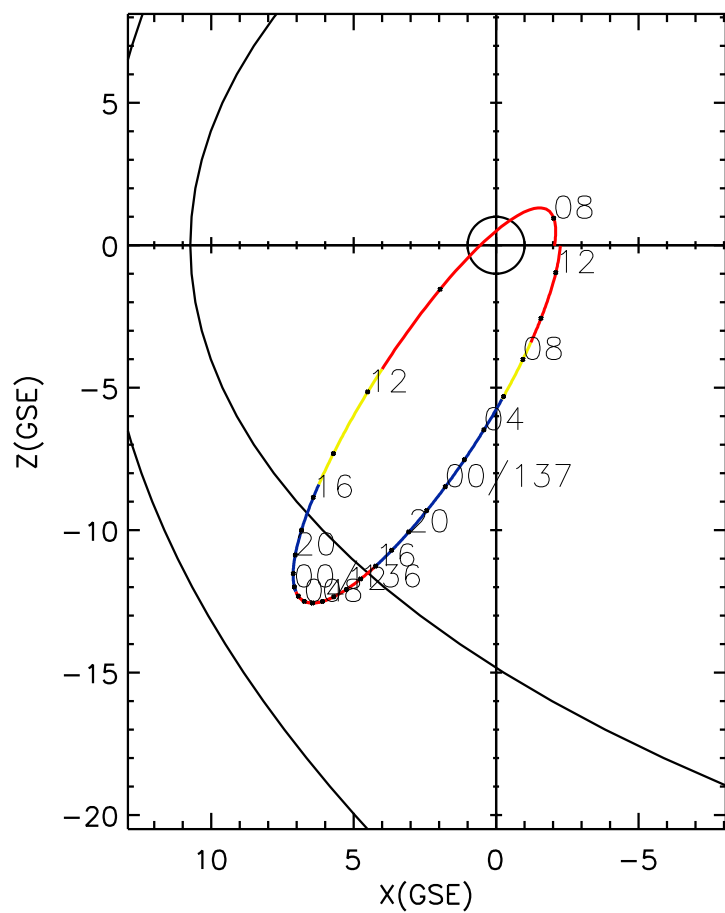
CLUSTER 2 orbit 2012 135 (05/14) 06:51 UT to 2012 137 (05/16) 13:06 UT
