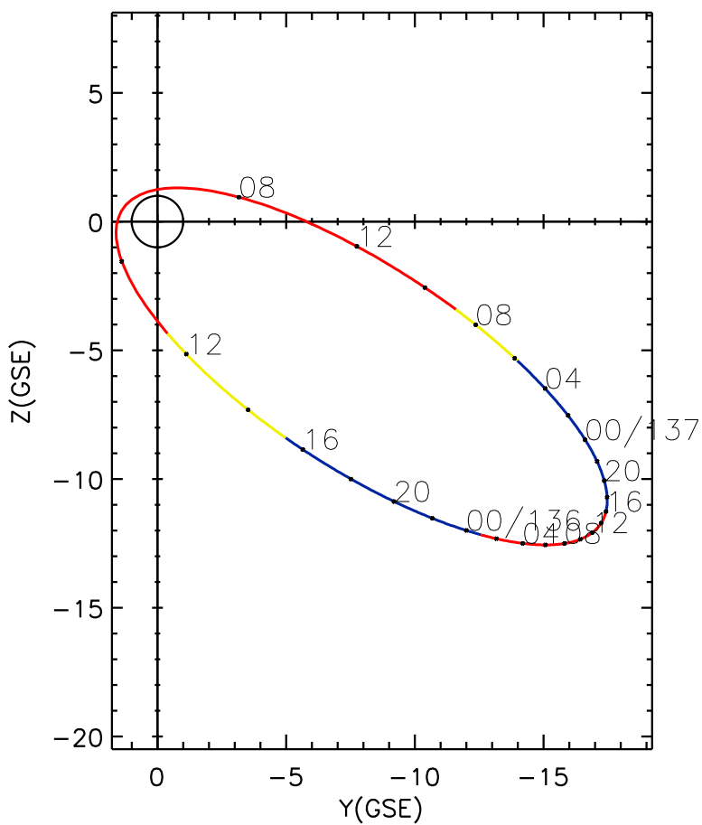
CLUSTER 2 orbit 2012 135 (05/14) 06:51 UT to 2012 137 (05/16) 13:06 UT
