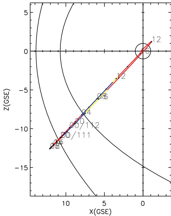
CLUSTER 2 orbit 2012 110 (04/19) 10:01 UT to 2012 112 (04/21) 16:16 UT
