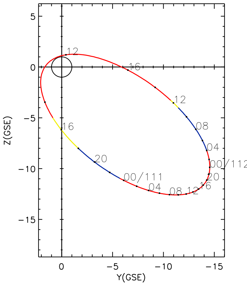
CLUSTER 2 orbit 2012 110 (04/19) 10:01 UT to 2012 112 (04/21) 16:16 UT
