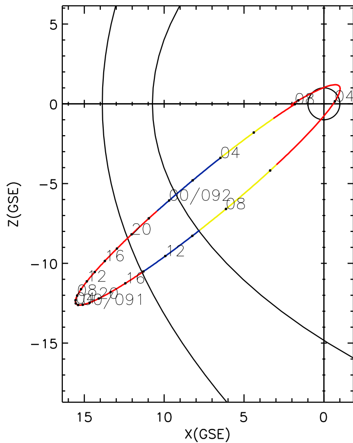
CLUSTER 2 orbit 2012 090 (03/30) 01:41 UT to 2012 092 (04/01) 08:01 UT
