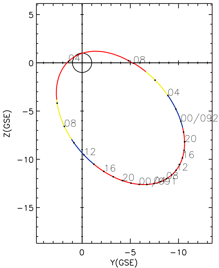
CLUSTER 2 orbit 2012 090 (03/30) 01:41 UT to 2012 092 (04/01) 08:01 UT
