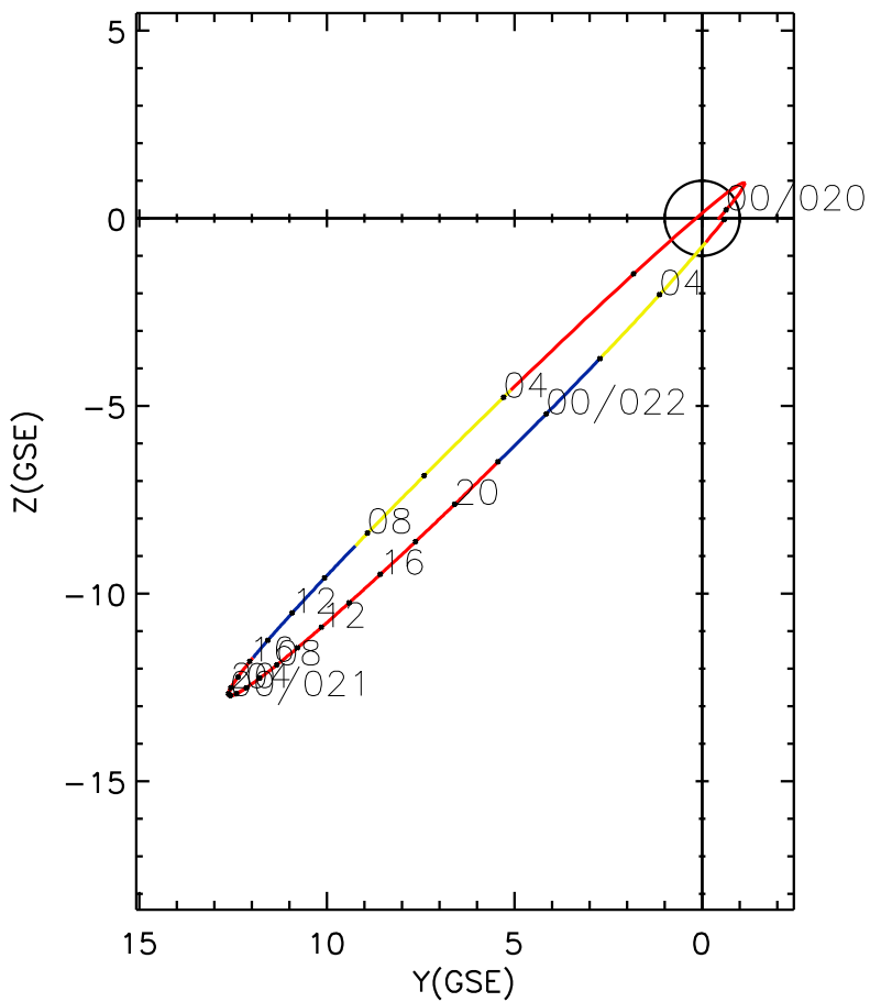
CLUSTER 2 orbit 2012 019 (01/19) 23:46 UT to 2012 022 (01/22) 06:01 UT
