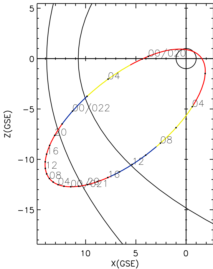
CLUSTER 2 orbit 2012 019 (01/19) 23:46 UT to 2012 022 (01/22) 06:01 UT
