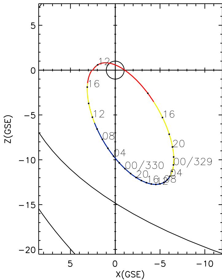
CLUSTER 2 orbit 2011 328 (11/24) 11:26 UT to 2011 330 (11/26) 17:41 UT
