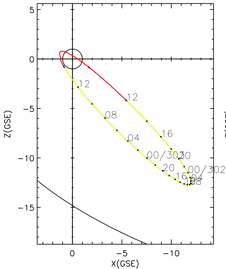
CLUSTER 2 orbit 2011 301 (10/28) 08:21 UT to 2011 303 (10/30) 14:36 UT
