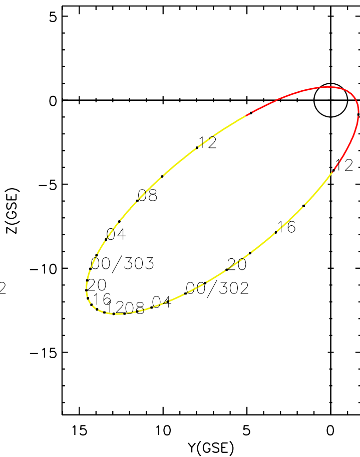
CLUSTER 2 orbit 2011 301 (10/28) 08:21 UT to 2011 303 (10/30) 14:36 UT
