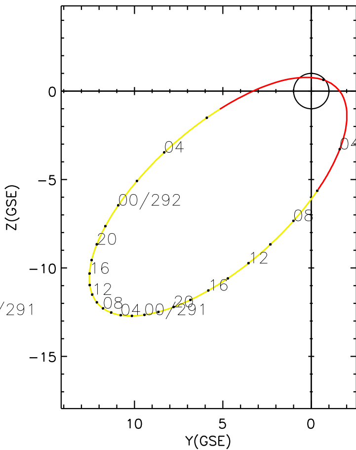
CLUSTER 2 orbit 2011 290 (10/17) 01:01 UT to 2011 292 (10/19) 07:16 UT
